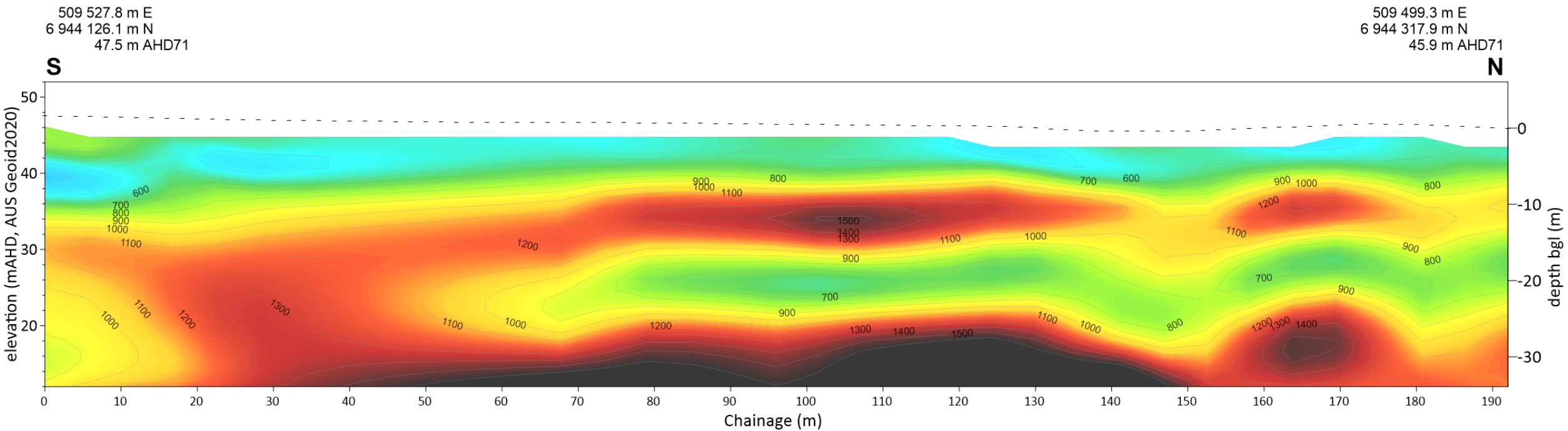
Seismic Line MASW AU-GP 121
